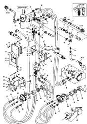
ETB-010470, Hydraulika Hydro II
