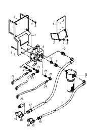
ETB-010479, Comfort - blok
